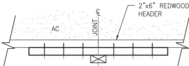
REDWOOD SPLICE - PLAN VIEW
