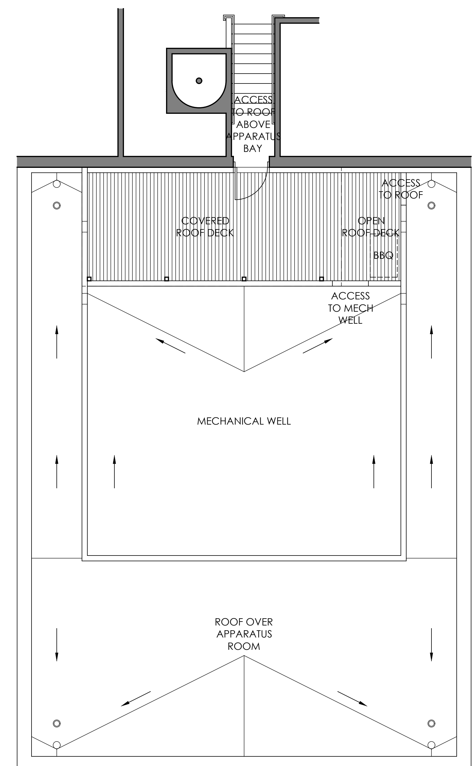
PROPOSED ROOFTOP
