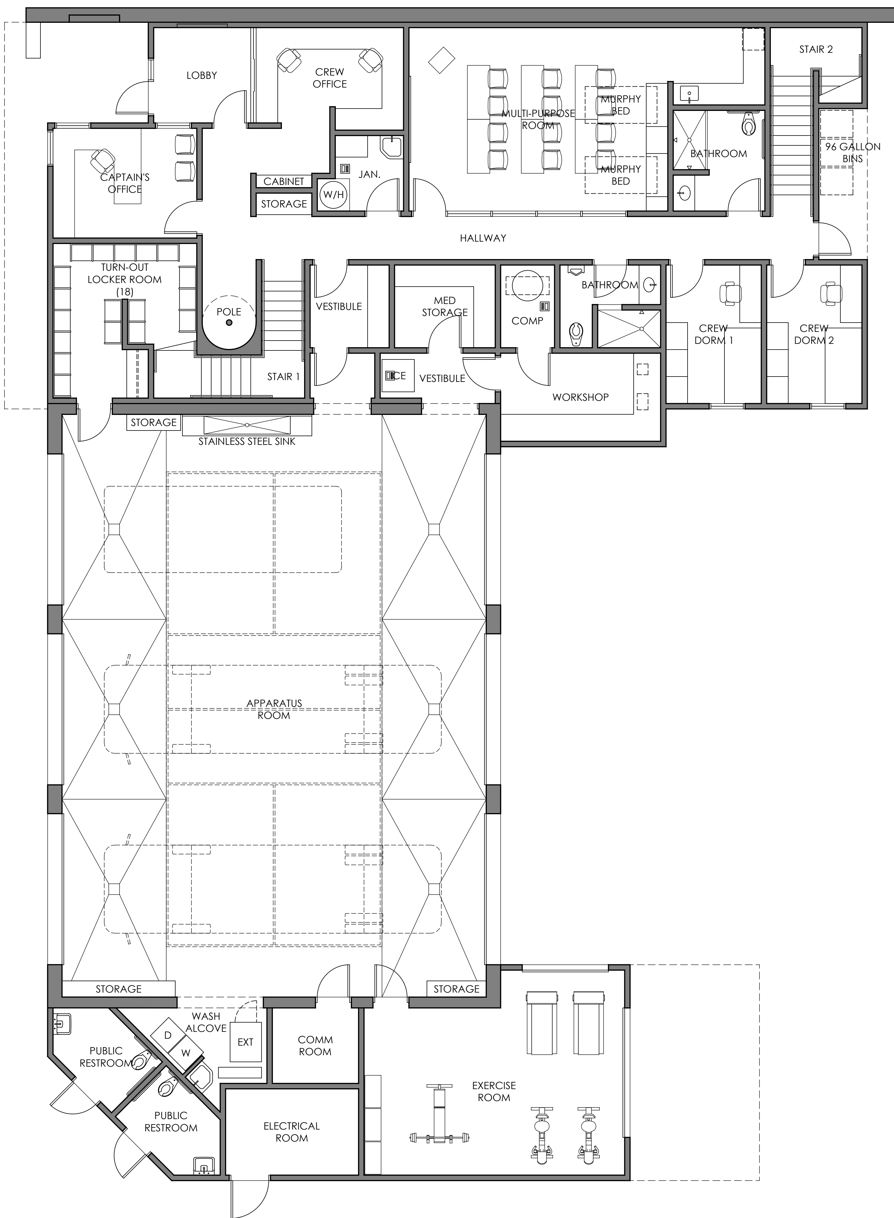
PROPOSED 1ST FLOOR 5,804 S.F.
