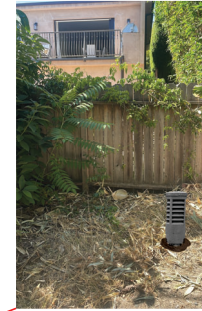
SCE VENT STANDPIPE 8" DIAMETER, 34" HEIGHT GRANITE (GRAY) FINISH
