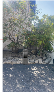
SCE VENT STANDPIPE 8" DIAMETER, 34" HEIGHT GRANITE (GRAY) FINISH
