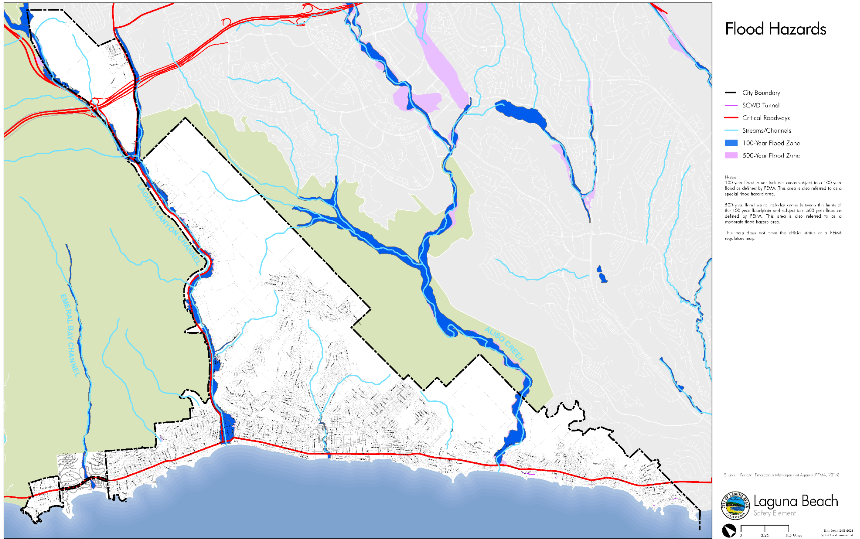
FIGURE S-6 – FLOOD HAZARDS
