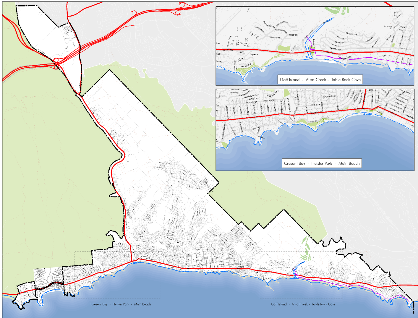
FIGURE S-7 – SEA LEVEL RISE
